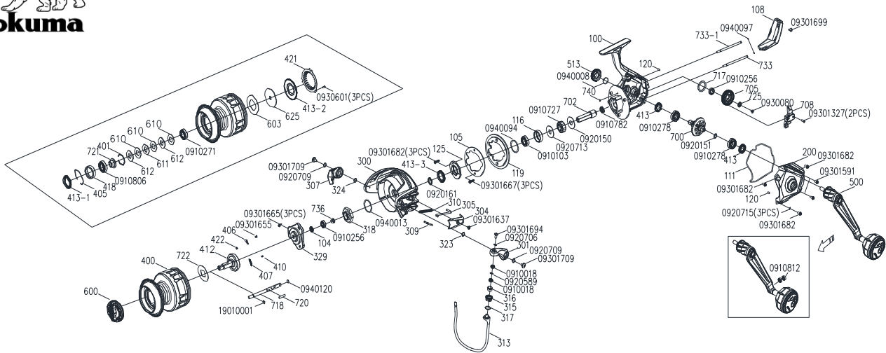
TSR-6000HA PARTS LIST
