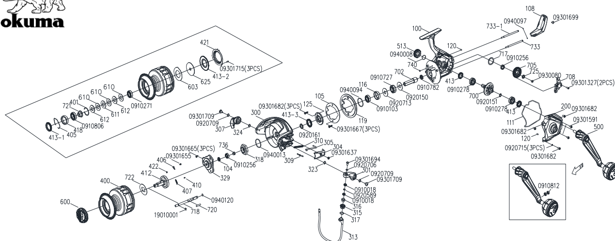
TSR-5000HA PARTS LIST
